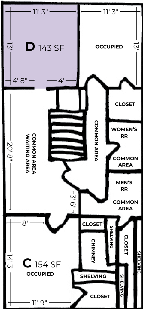
SECOND FLOOR
