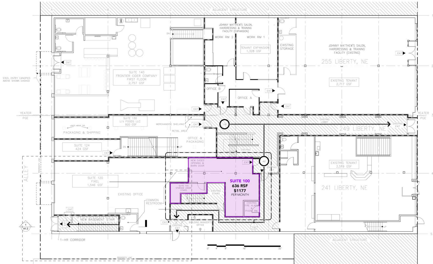
1 GROUND FLOOR PLAN 1/8" = 1'-0"
